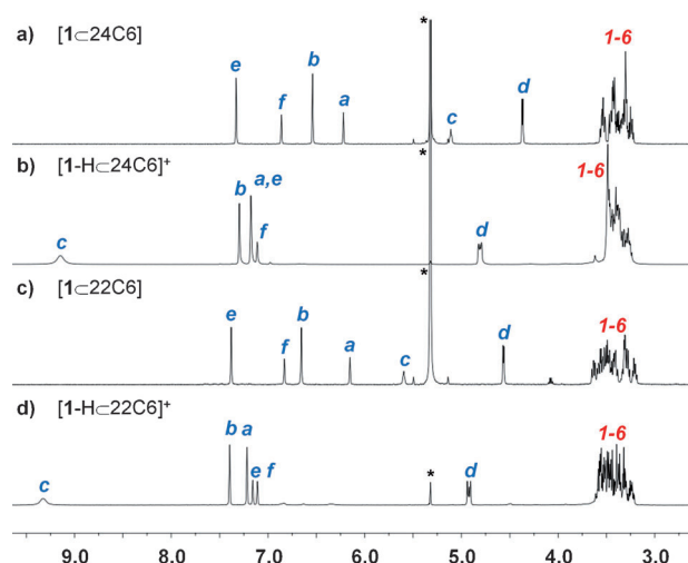
Figure 3. ^1H NMR spectra (500 MHz, CD_2Cl_2 , 298 K) of a) [1C24C6], b) [1-HC24C6] ^+ (product of the reaction of [1C24C6] with B(C_6F_5)_3 and H_2(g) ), c) [1C22C6], and d) [1-HC22C6] ^+ (product of the reaction of [1C22C6] with B(C_6F_5)_3 and H_2(g) ).
