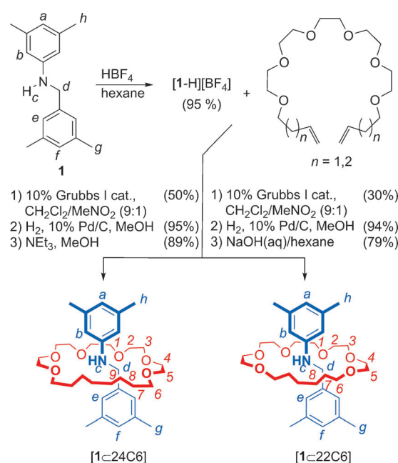
Scheme 1. Synthesis of [2]rotaxanes [1<24C6] and [1<22C6] by the clipping method converts the aniline base 1 into sterically hindered MIM bases by restricting access to the Lewis basic nitrogen atom.
