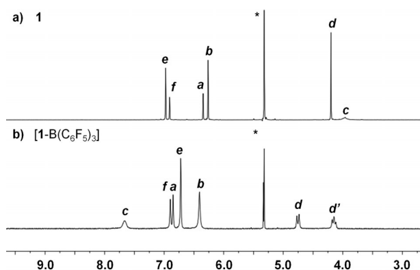
Figure 2. 1 H NMR spectra (500 MHz, CD 2 Cl 2 , 298 K) of a) the aniline 1, and b) the adduct [1-B(C 6 F 5 ) 3 ].
