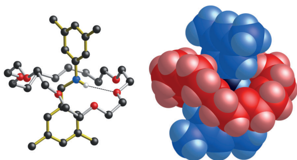
Figure 1. Left: ball-and-stick representation of the X-ray structure of [1⊂24C6]. Only the amine H atom involved in H bonding is shown, all others are omitted for clarity. Right: space-filling model of the same view with all H atoms showing the axle in blue and the macrocyclic wheel in red. The aniline N atom colored dark blue is barely visible.
