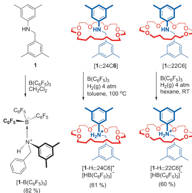
Scheme 2. Reactions of 1, [1⊂24C6], and [1⊂22C6] with Lewis acid B(C 6 F 5 ) 3 in the presence of H 2 (g).
